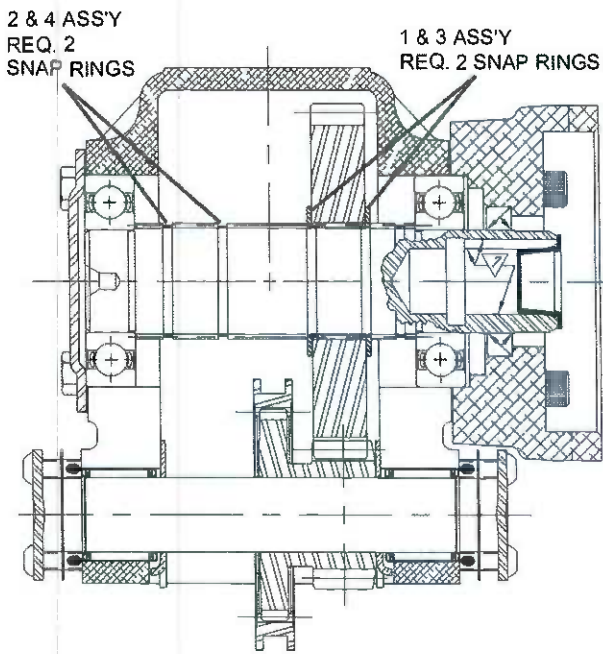
OUTPUT RATIO 04-13 HYDRAULIC TYPE SHAFT
