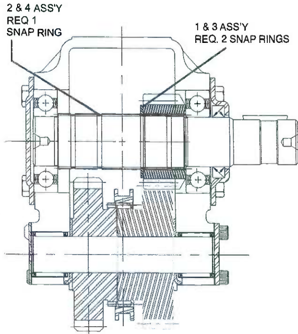
OUTPUT RATIO 15 & 18 REMOTE TYPE SHAFT
