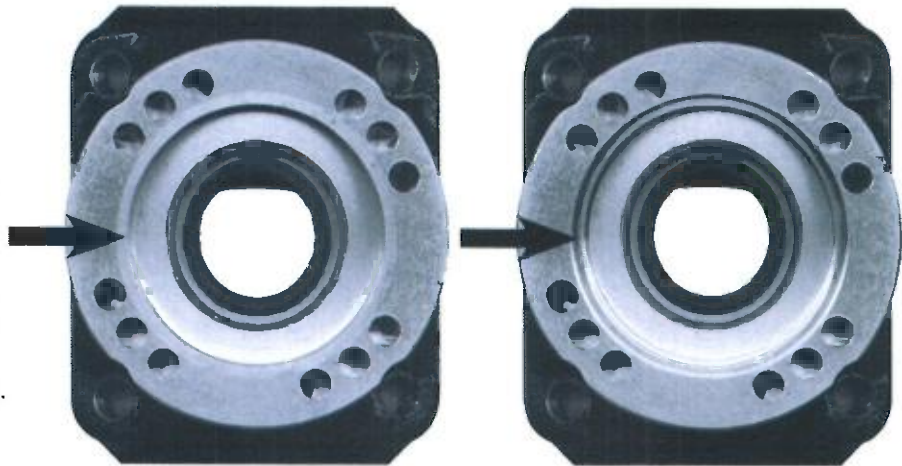
NO GROOVE IN FLANGE (USE 13T38542 GASKET)
