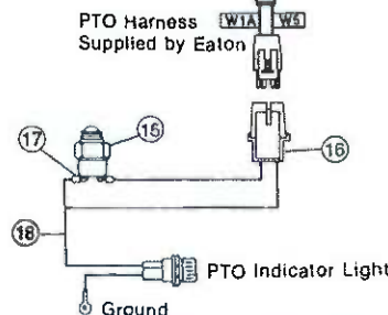
Eaton Fuller Transmission Electrical Connector
