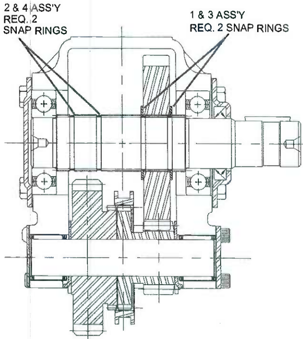
OUTPUT RATIO 04-13 REMOTE TYPE SHAFT
